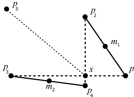
Figure 5.3: Construction Used in the First Proof of Lemma 5.1
