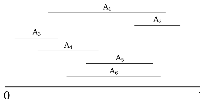
Figure 4.1: Linear Graph of a (2, 3, 6) -Society
