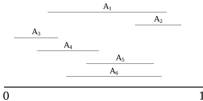
Figure 3.2: Linear Graph of a (2, 3, 6) -Society
