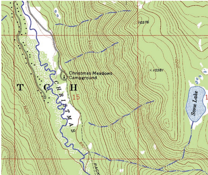
Fig. 4.2 Topographic map near Christmas Meadows Campground, Utah. Note that the river lines run orthogonal to the level curves, providing a demonstration of the steepest descent flow. (Courtesy of Topozone, www.topozone.com .)
