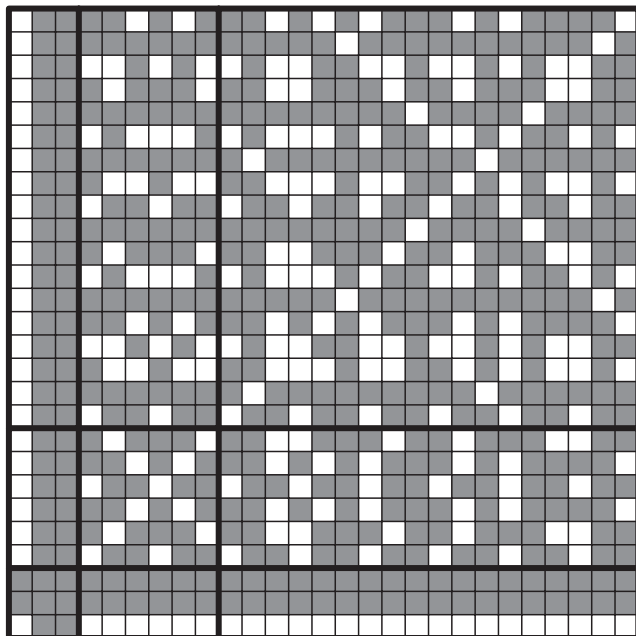
Figure 2 Every solid rectangle, except for the one in the lower left corner, has twice as many dark squares (representing relatively prime polynomials in \mathbb{Z}_3[x] ) as light squares. But how do you assign two dark squares to each light square?
