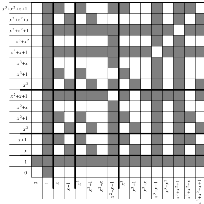
Figure 1 In every solid rectangle, except for the one in the lower left corner, half of the polynomials in \mathbb{Z}_2[x] are relatively prime (as represented by the dark squares). But how do you pair up the dark squares with the light squares?
